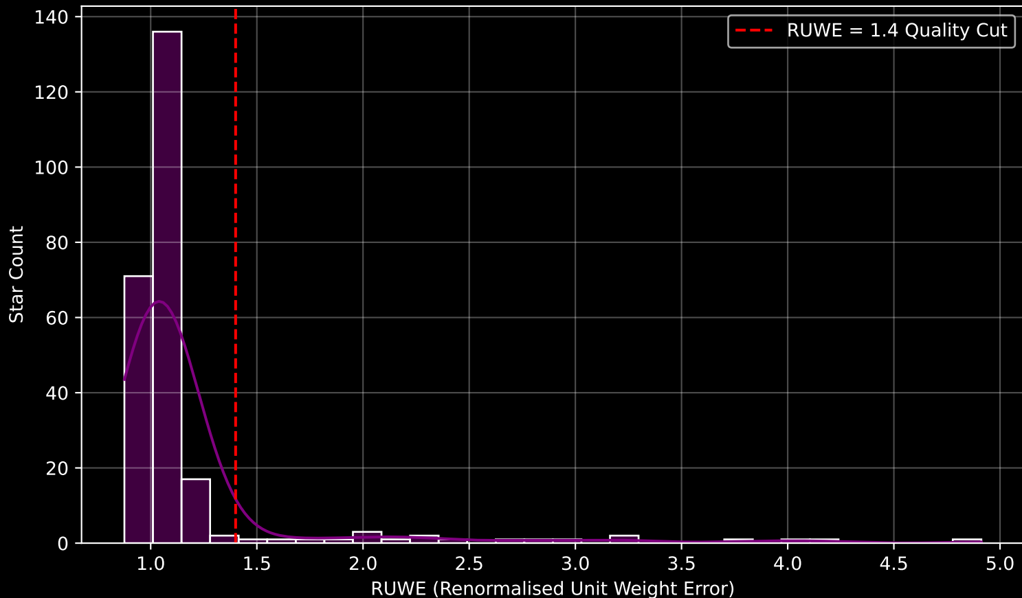
GAPOGEE DR17 Field [LAMBDAORI-B] RUWE Distribution (n= 246)
