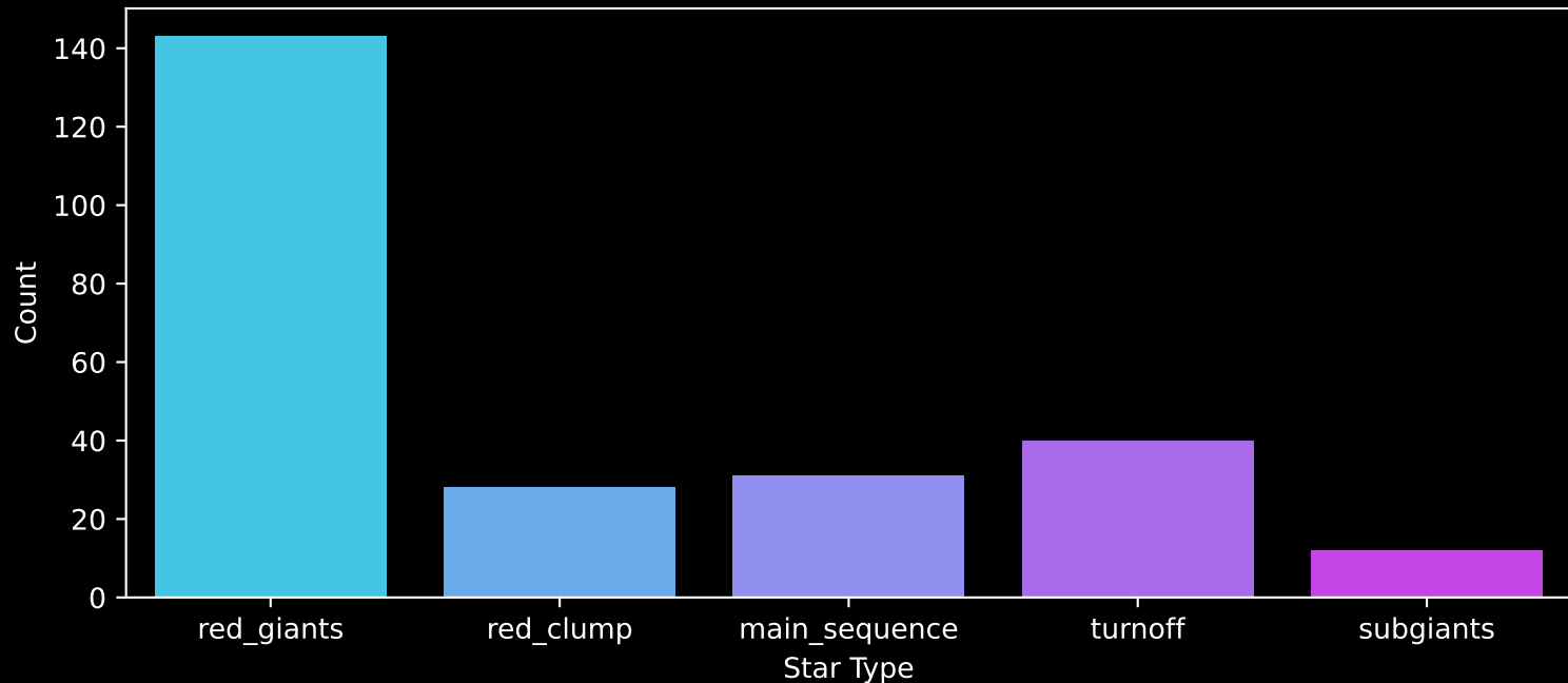
APOGEE DR17 Field: [LAMBDAORI-B] Count plot of Star Type
