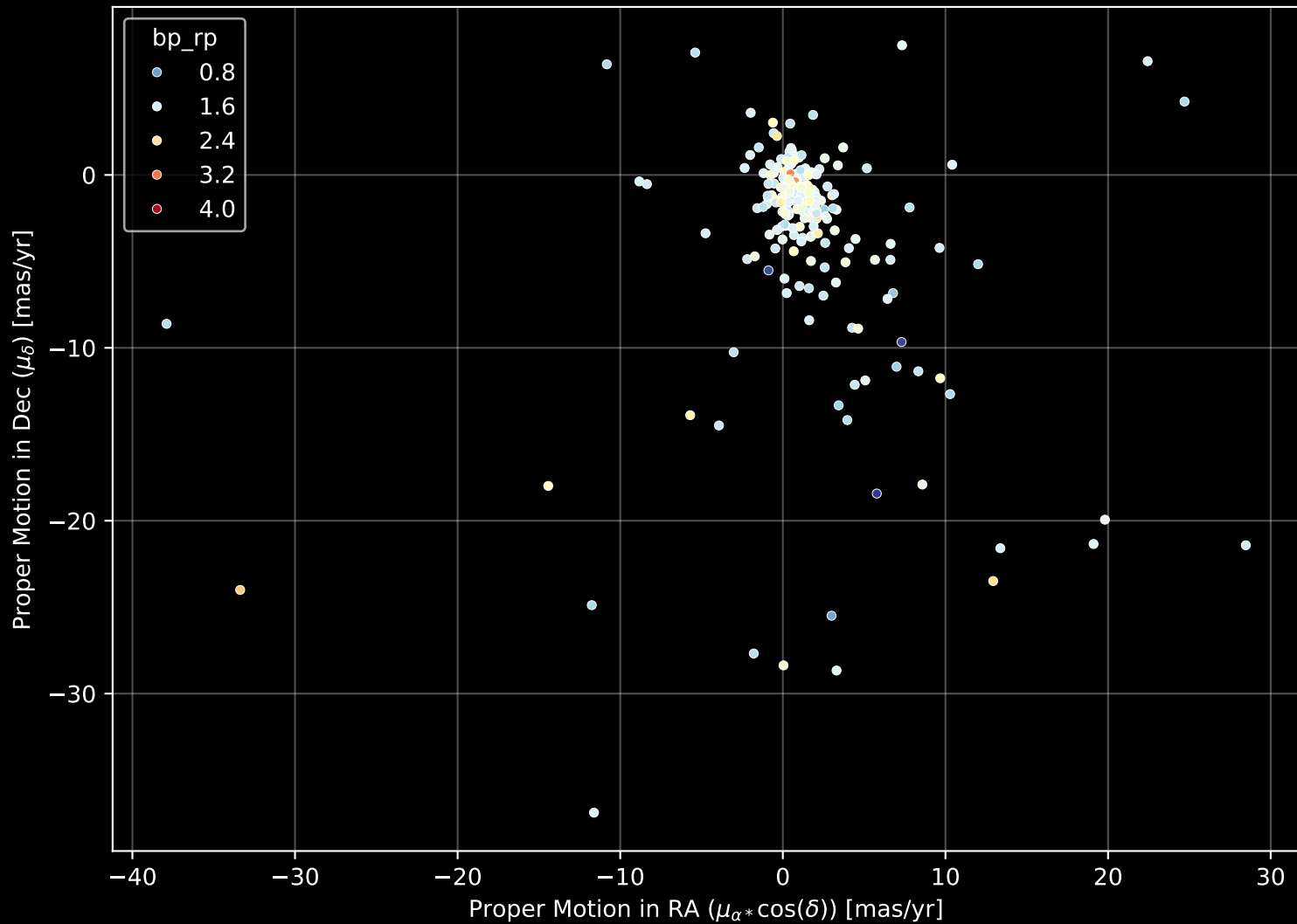
APOGEE DR17 Field: [LAMBDAORI-B] Proper Motion Diagram (n= 254)
