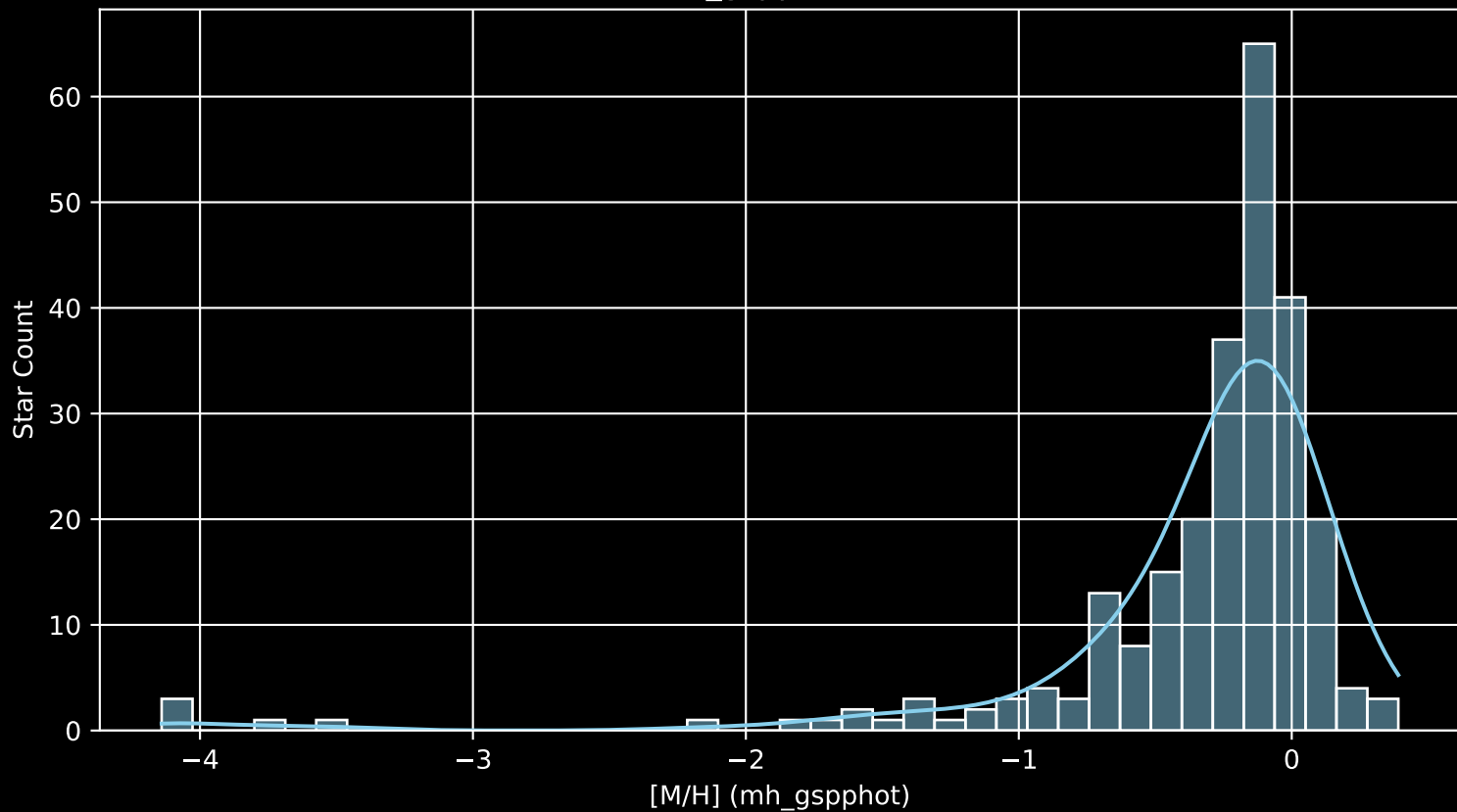
APOGEE DR17 Field: [LAMBDAORI-B [M/H] (mh_gspphot) (n= 253)
