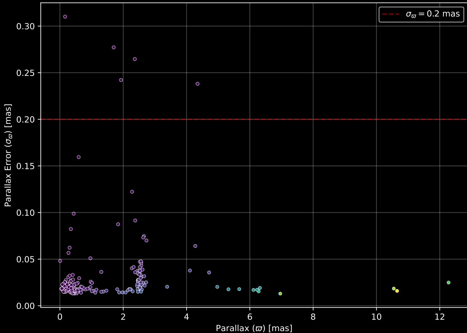
APOGEE DR17 Field: [LAMBDAORI-B] Parallax Quality (n= 254)
