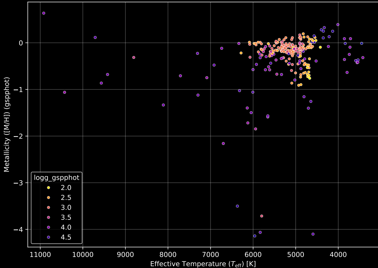
APOGEE DR17 Field: [LAMBDAORI-B] Stellar Population Parameters (n= 254)
