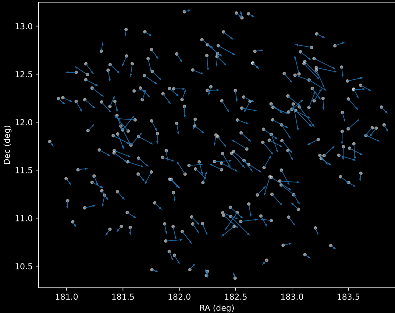
APOGEE DR17 Cluster 0 Proper Motion Vectors (n=213)
