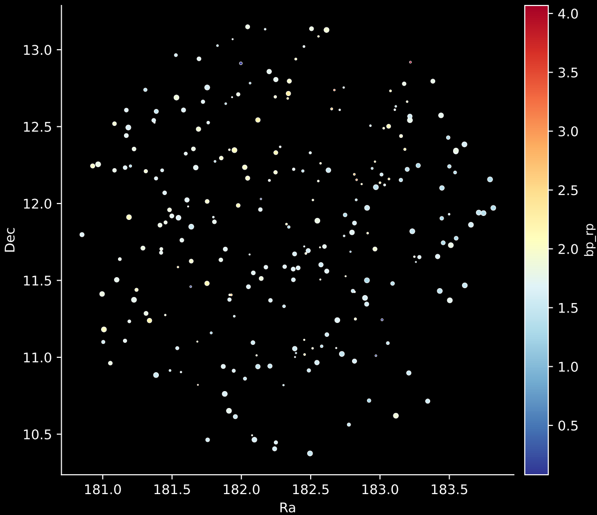
APOGEE DR17 Field: [LAMBDAORI-B] Stars: 254
